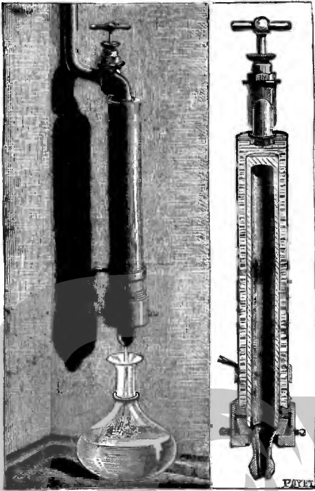
Filter developed in 1884 by bacteriologist Charles Edouard Chamberland (1851-1908). The liquid is pumped through a porcelain filter component. Source: www.gutenberg.org/dirs/1/1/1/7/3/11734/11734-h/illustrations/4a.png , retrieved 22 June 2005.
