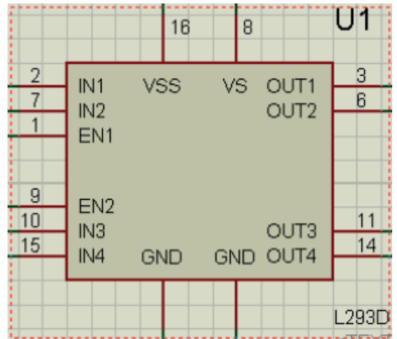
Figure 18 – Driver L293D
