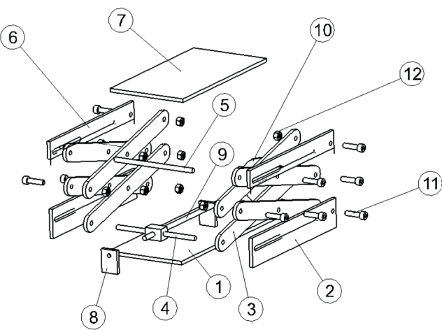
Figure 2 – Elevating scissor platform model exploded view
