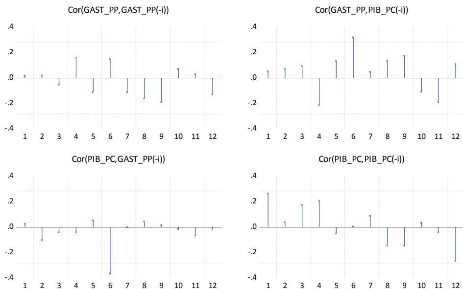
Figura 17. Test residual-correlograma
