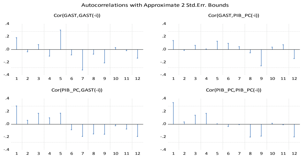
Figura 15. Test residual-correlograma
