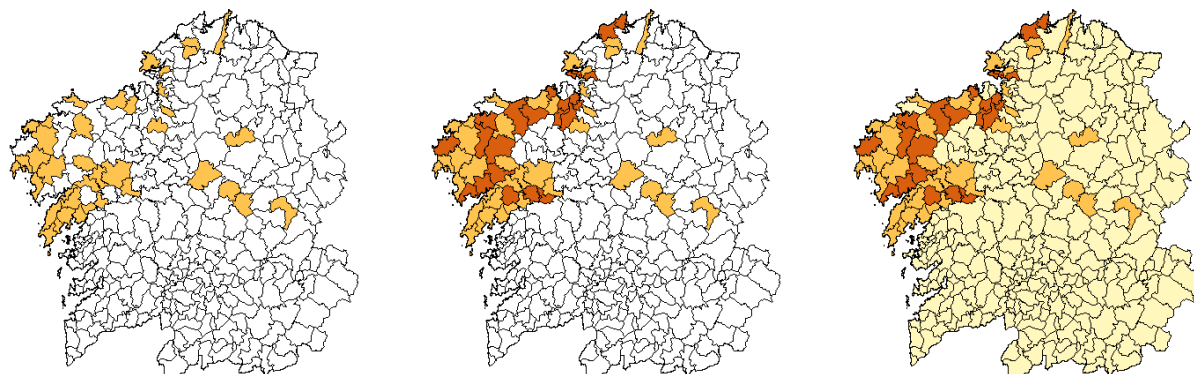
Figura 9.2: Left: councils for \tau = 0.8 (left connected components - Figure 9.1). Middle: councils for \tau = 0.8 (left and right connected components - Figure 9.1). Right: all councils in Galicia.
