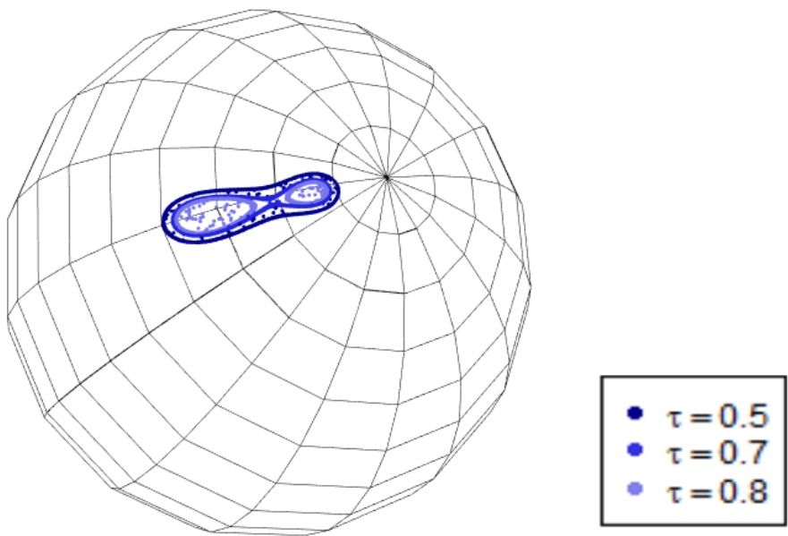
Figura 9.1: HDiR from toponymic, patronymic and apelative surnames.
