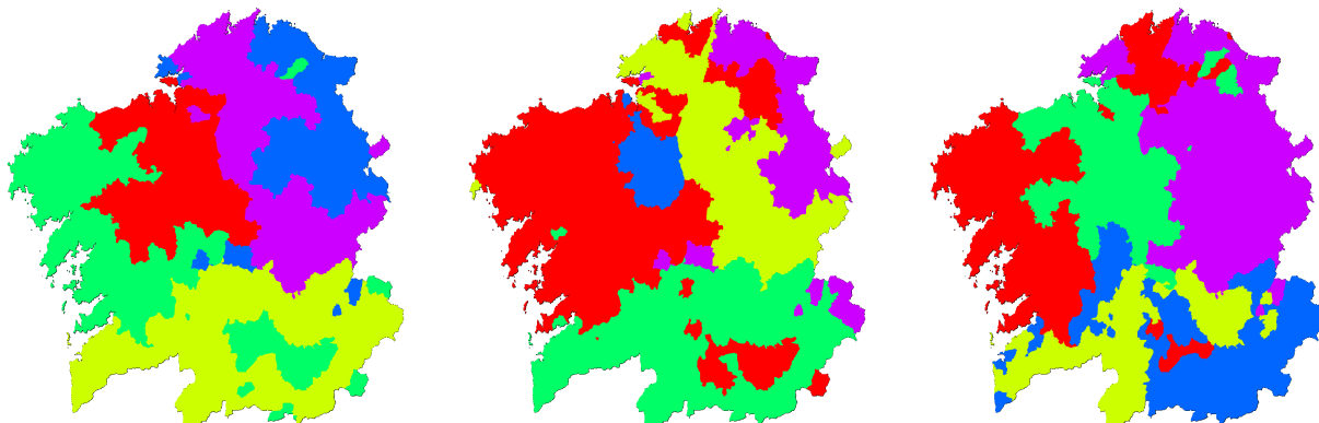
Figura 9.3: Spherical cluster results considering all data (left); Spherical cluster results filtering by population born before 1965 (center); Spherical cluster results filtering by population born before 1945 (right).
