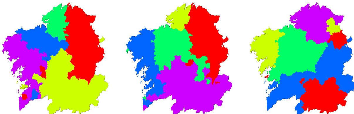
Figura 9.4: Spherical cluster results considering all data (and removing those ones below and above the 5% and 95% quantiles of the distribution of number of councils) (left); Spherical cluster results filtering by population born before 1965 (and removing those ones below and above the 5% and 95% quantiles of the distribution of number of councils) (center); Spherical cluster results filtering by population born before 1945 (and removing those ones below and above the 5% and 95% quantiles of the distribution of number of councils) (right).
