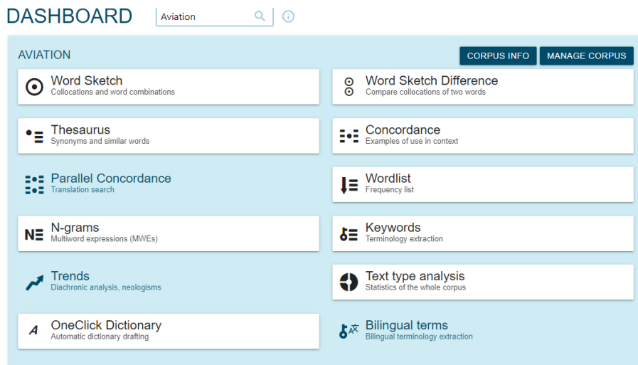
Figure 1: SketchEngine tools.
