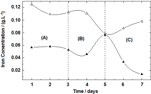
Figure 9- Variations in the concentration of \text{Fe}^{2+} (Δ) and \text{Fe}^{3+} (▲), in the continuous growth of Mesophilic Microorganisms, as the flow of nutrients increases: (A) 3.4 L/day; (B) 5.67 L/day and (C) 17.0 L/day.
