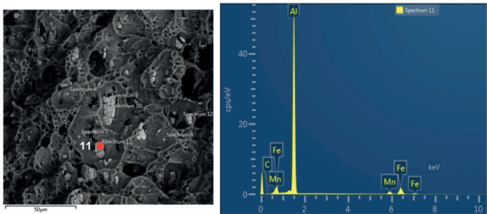
Figura 24: Spectrum 11.
