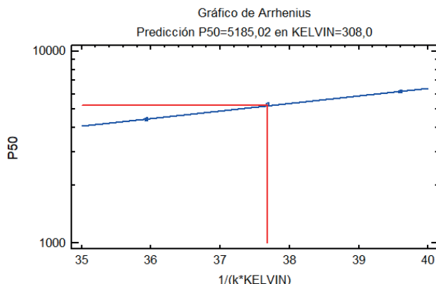
Figure 2 Arrhenius plot
