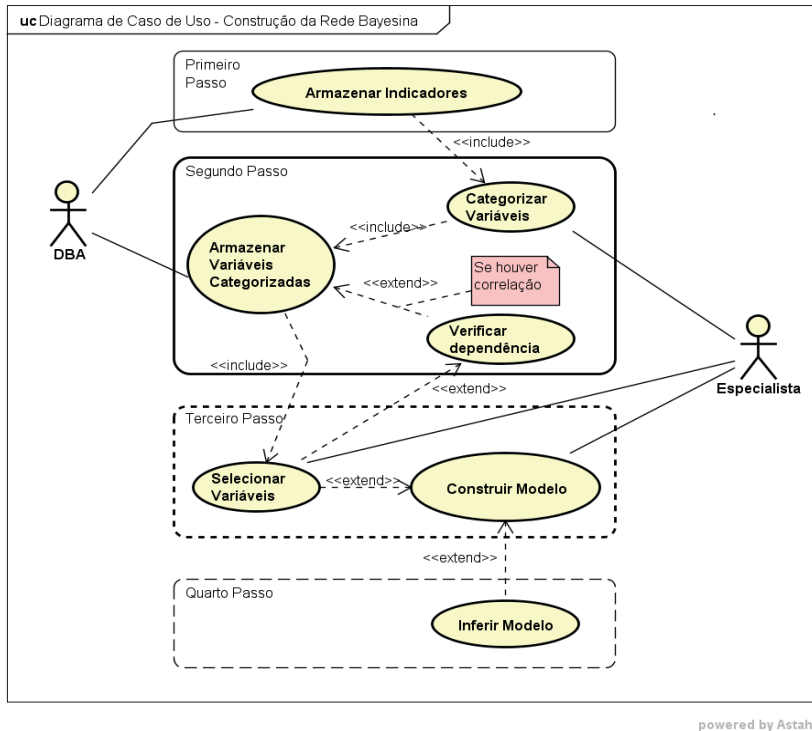
Figure 4 – Use Case Diagram. Source: Calderaro (2016).
