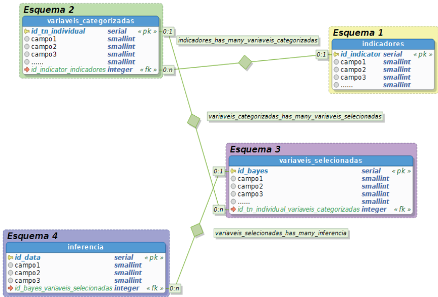
Figure 7 – Database structure. Source: Calderaro (2016).
