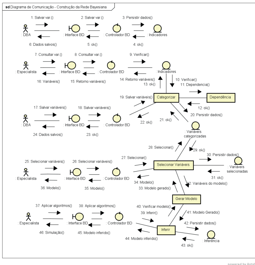
Figure 6 – Communication Diagram. Source: Calderaro (2016).
