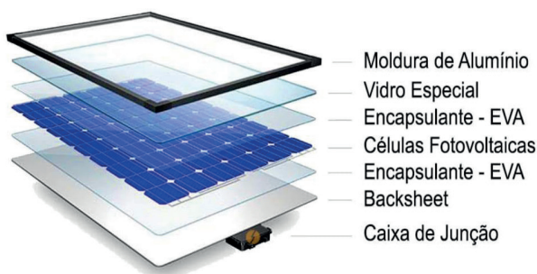
Figura 1: Painel solar
