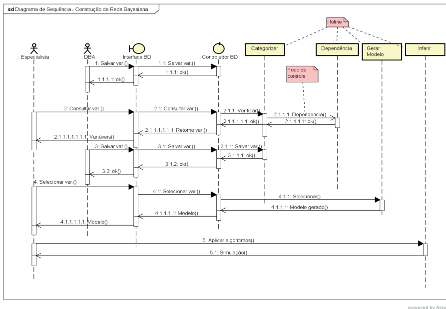
Figure 5 – Sequence Diagram. Source: Calderaro (2016).
